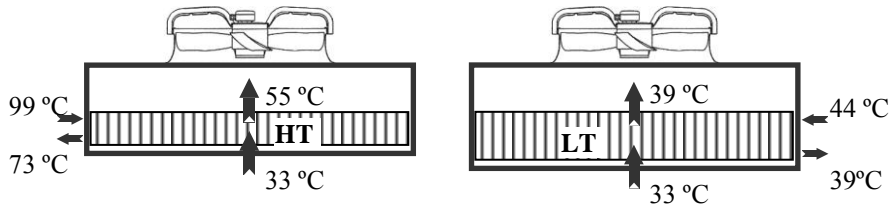
Picture 2. The cooling of HT (Jacket Water) and LT (After Cooler) circuits with separate dry coolers
